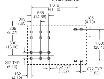
Suggested PC Board Layout (Bottom View)
