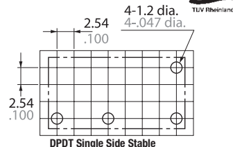
DPDT Single Side Stable
